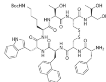
[Lys 5 (Boc)]lanreotide acetate
