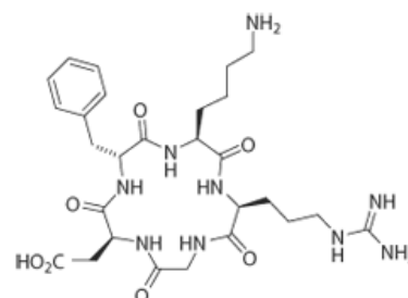
Cyclo-RGDfK
